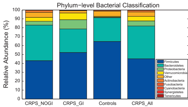
Fig. 2. The relative abundance of the bacterial composition, seen at the phylum level. Participants with CRPS show a reduction in Firmicutes and increased levels of Proteobacteria. The CRPS_GI ( n = 5 ) contains CRPS subjects that expressed GI issues, the CRPS_NOGI are comprised of CRPS subjects sans GI complications, the CRPS_All group is a cohort of all the CRPS subjects. Verrucomicrobia appears elevated in the CRPS groups, however the Student's t-test did not produce significant results. Further inspection revealed the phylum's increased levels can be attributed to a few CRPS subjects.
