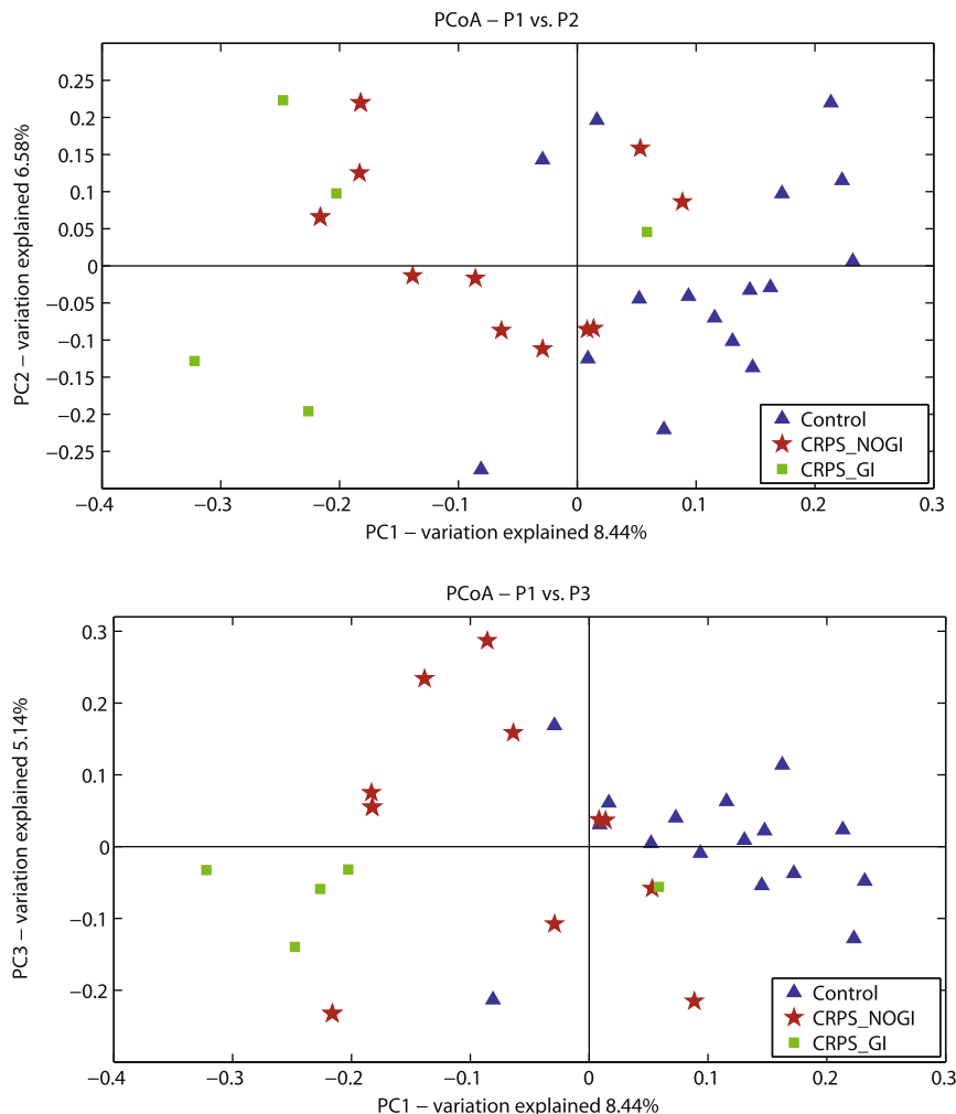
Fig. 3. Principal coordinate analysis (PCoA) generated from the unweighted UniFrac matrix of OTUs of CRPS subjects with gastrointestinal difficulties (CRPS_GI, n = 5 ), CRPS study participant's with no gastrointestinal difficulties (CRPS_NOGI, n = 11 ), and health controls (controls, n = 16 ).
