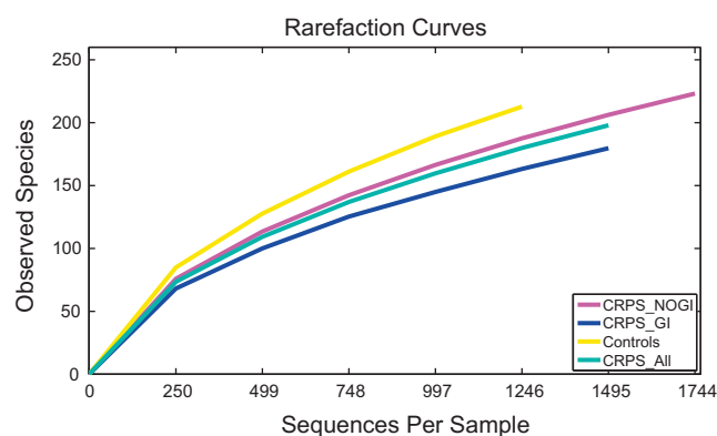
Fig. 1. Rarefaction analysis of V2-targeted pyrosequenced reads of the bacterial 16S rRNA gene recovered from human fecal specimens. The rarefaction curves were constructed at 97% (species level) sequence similarity and were pooled together according to disease group specification.
